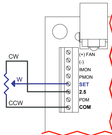
Figure 18. External setpoint adjustment.
