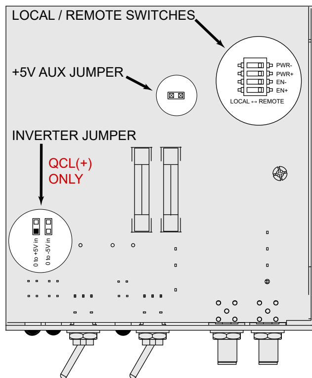
Figure 4. Inverter Jumper Location
