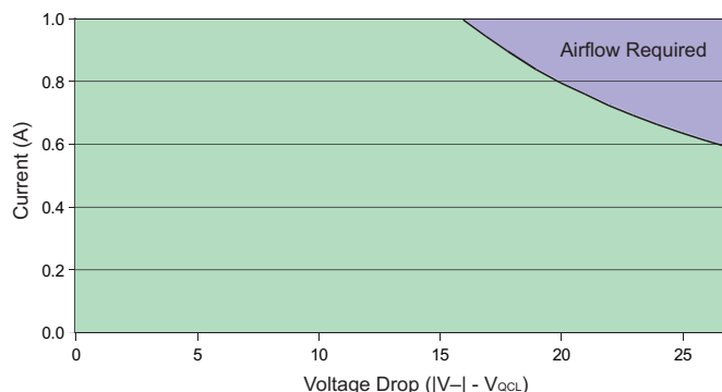
Figure 16. QCL1000(+) SOA Chart, at 25°C
