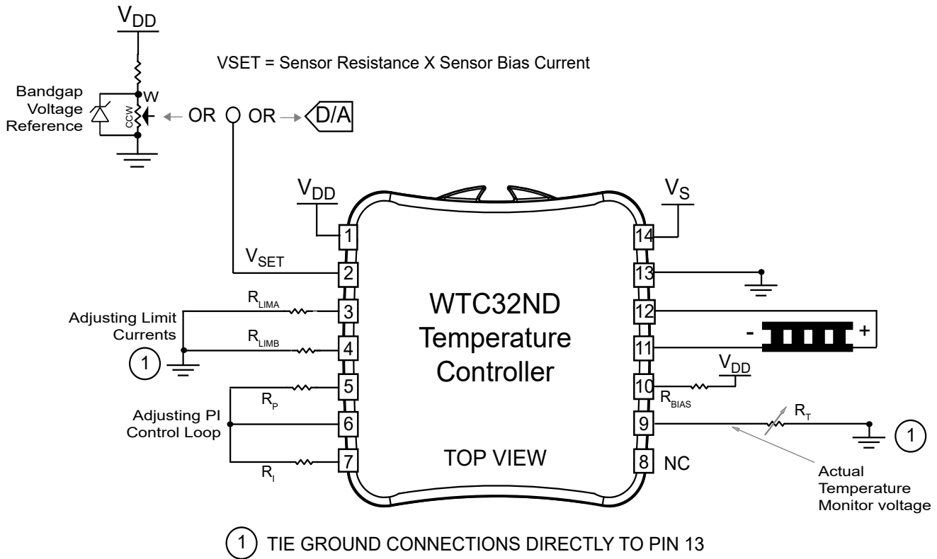
Figure 3. WTC32ND Quick Connect for TEC with Thermistor
