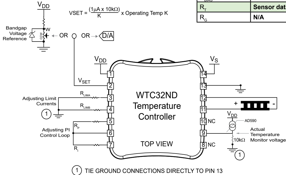
Figure 22. AD590 / Thermoelectric Operation -- Top View
