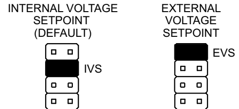
Figure 10. External and Internal Setpoint Jumpers
